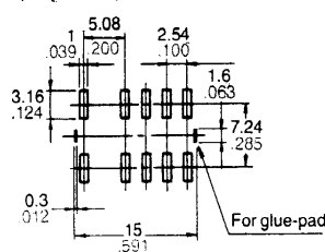
Suggested mounting pad (Top view)
